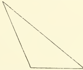
TRIANGLE HAVING AN OBTUSE ANGLE AND THREE UNEQUAL SIDES.
